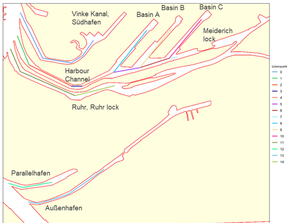
Figure 3: Segments of NO x line sources for ships sailing in the port of Duisburg
