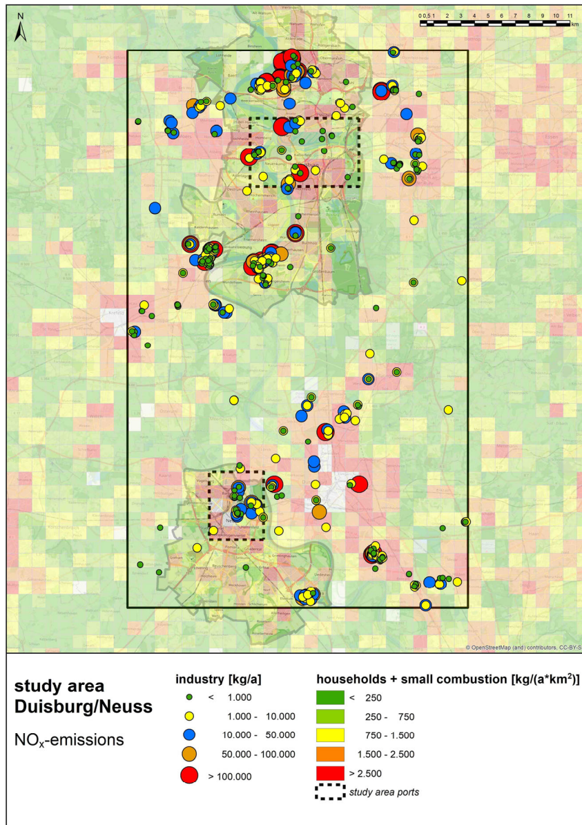
Figure 19: NO x emitters from industry and small combustion plants (HuK) in the study area, analysis year 2018
