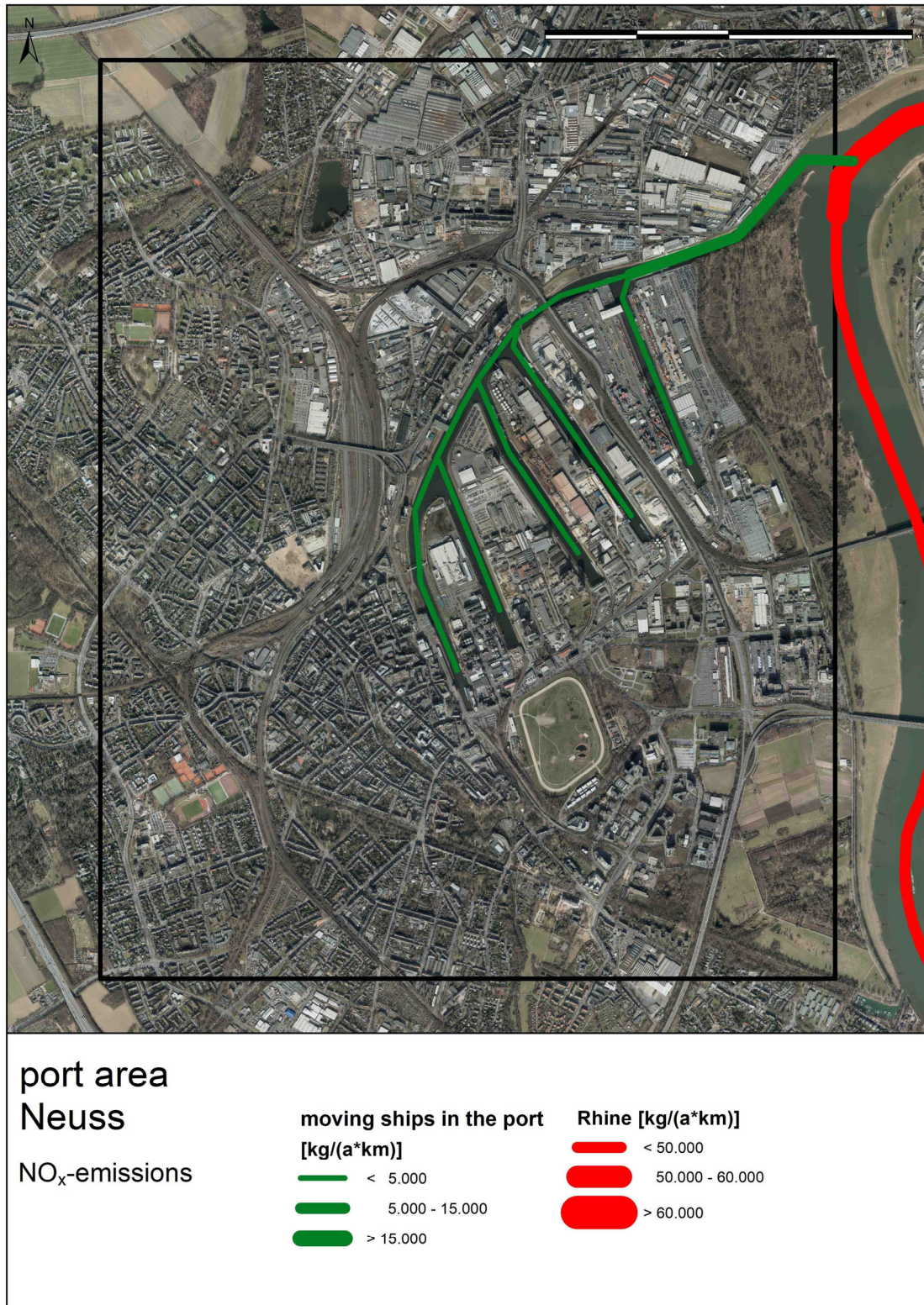
Figure 6: NO x emission densities of moving ships in the Neuss/Düsseldorf study area Inner box: Boundary of the port area
