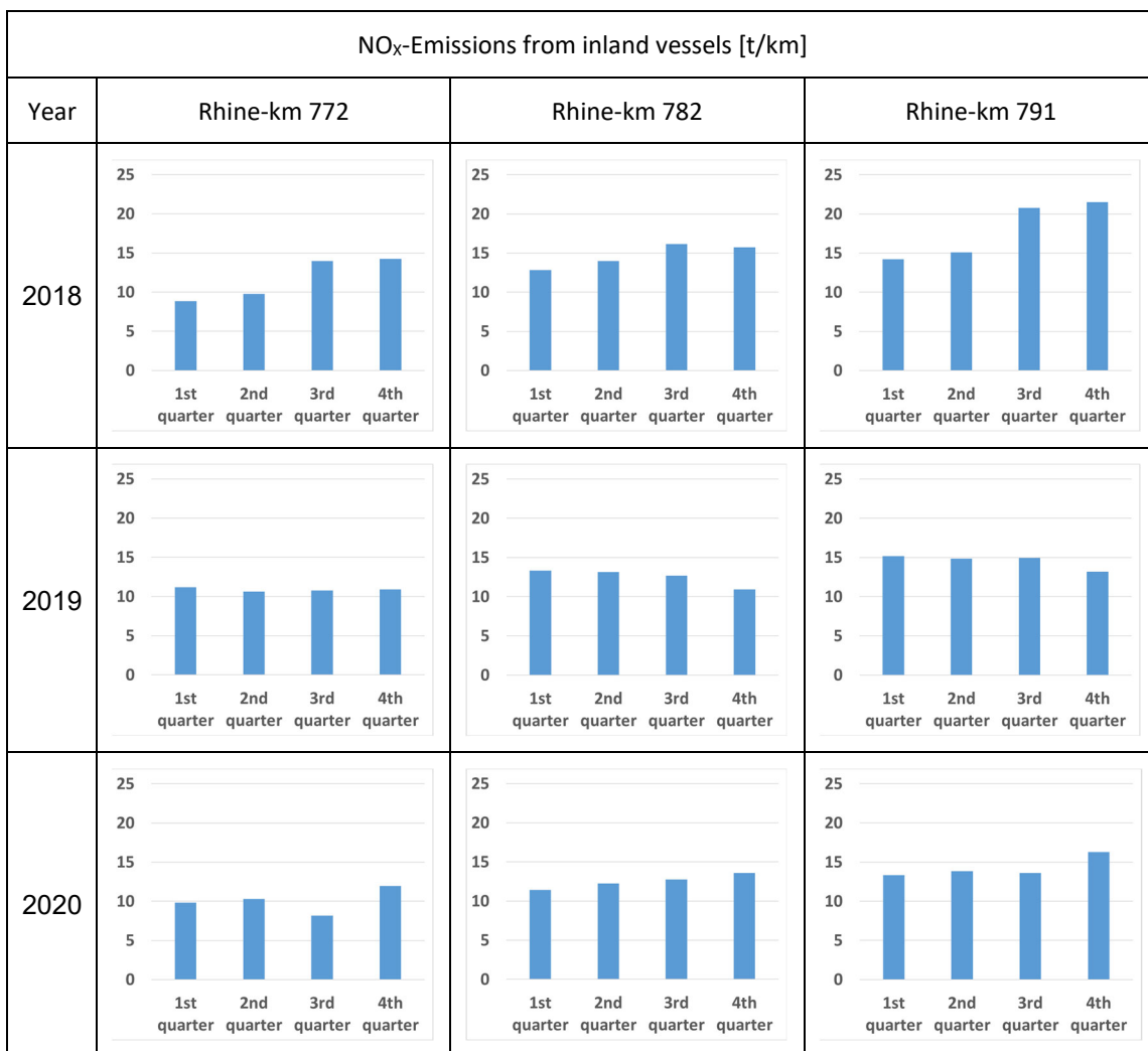
Figure 1: NO x -Emissions per quarter over the course of the year in the Duisburg section of the Rhine. The measuring station DURH is located at Rhine-km 782.
