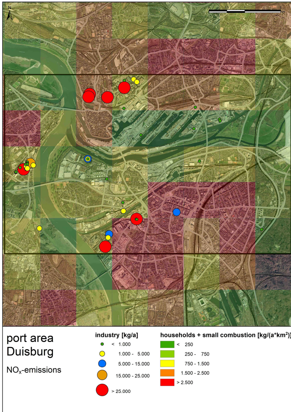
Figure 27: Annual NO x -emissions from industrial sources, small combustion plants and domestic furnaces in the Duisburg port area, analysis year 2018
