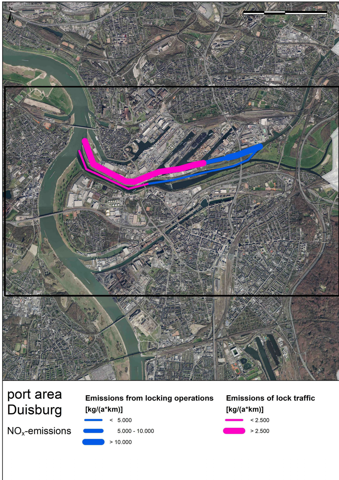
Figure 5: NO x emission densities of the ships travelling to the locks and the lock operations in the Duisburg study area. Inner box: Boundary of the port area
