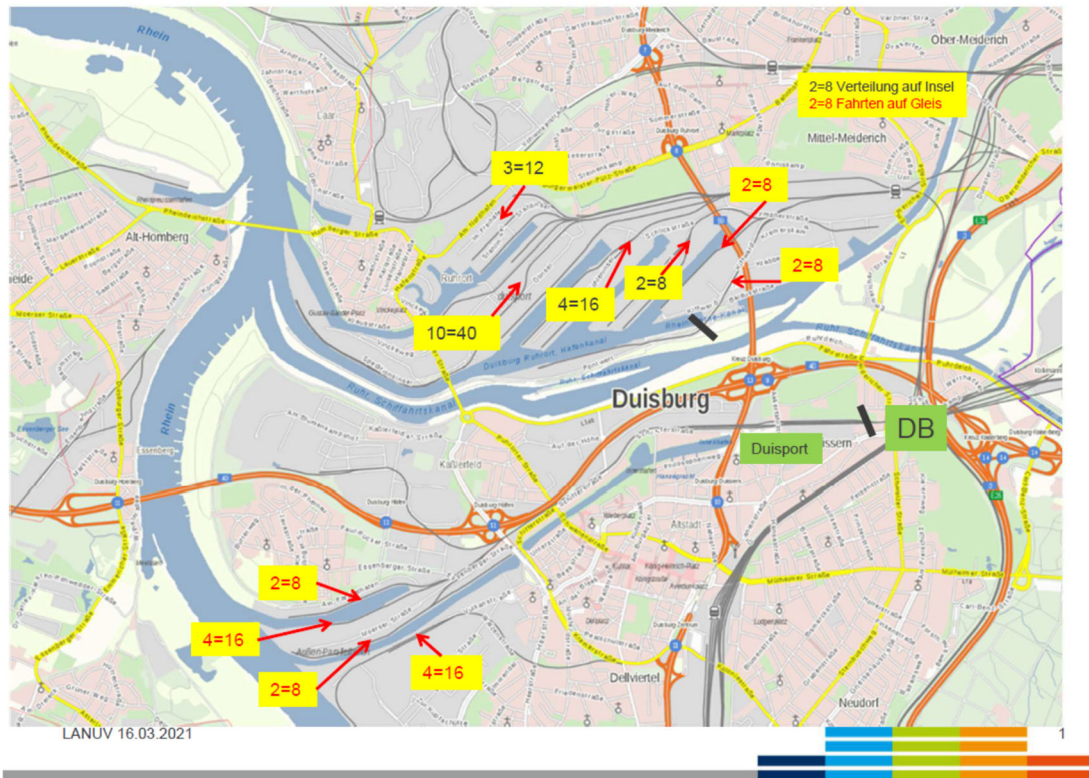
Figure 33: Number of trips of the locomotives of the Duisport port railway according to the port operators.
