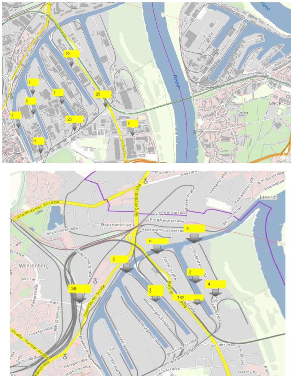
Figure 34: Number of trips of the locomotives of the Rheincargo port railway in the port of Neuss according to the port operators.
