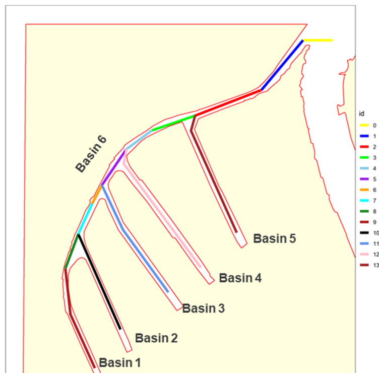
Figure 2: Segments of NO x line sources for ships sailing in the port of Neuss
