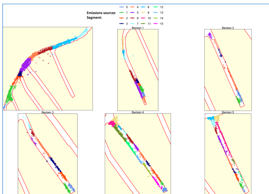
Figure 10: Allocation of the point data of the individual ships to the respective line sources (Port of Neuss).
