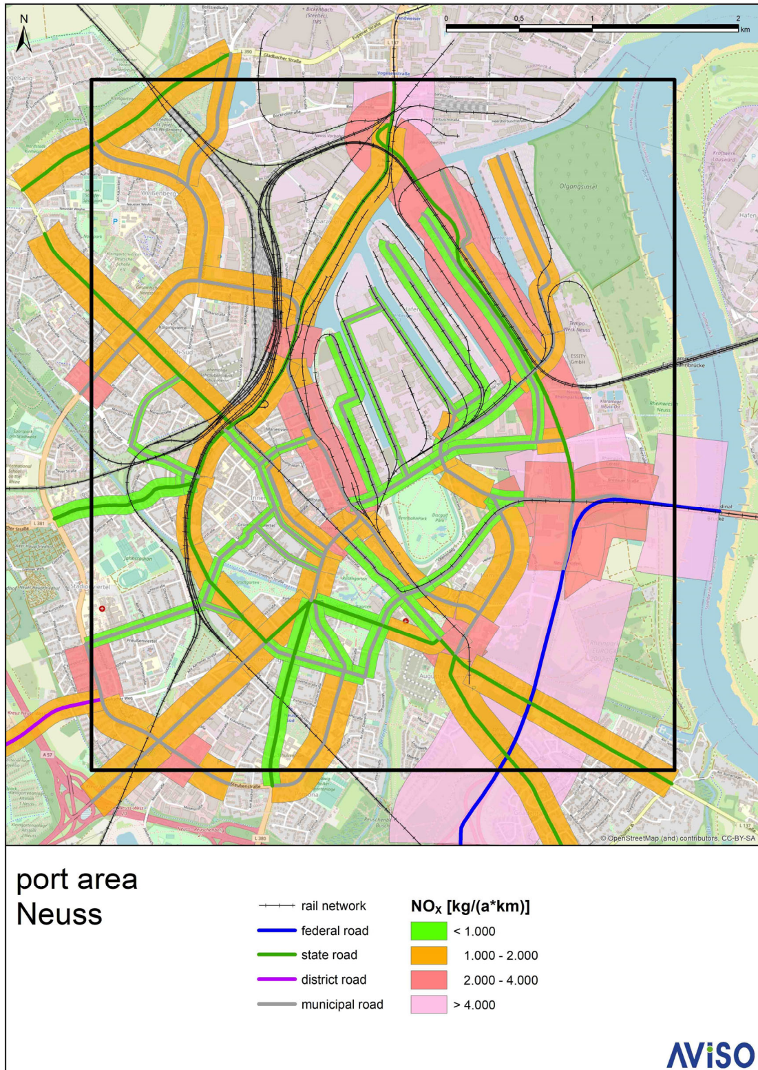
Figure 25: Annual NO x emissions from road traffic in the Neuss port area, analysis year 2018
