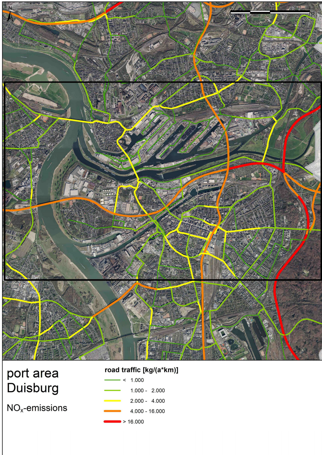
Figure 29: Annual NO x emissions from road traffic in the Duisburg port area, analysis year 2018
