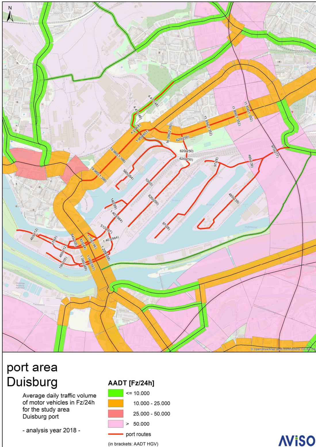
Figure 22: Motor vehicle traffic volumes in the port area for the analysis year 2018 (AADT=daily traffic volume, vehicles per day).
