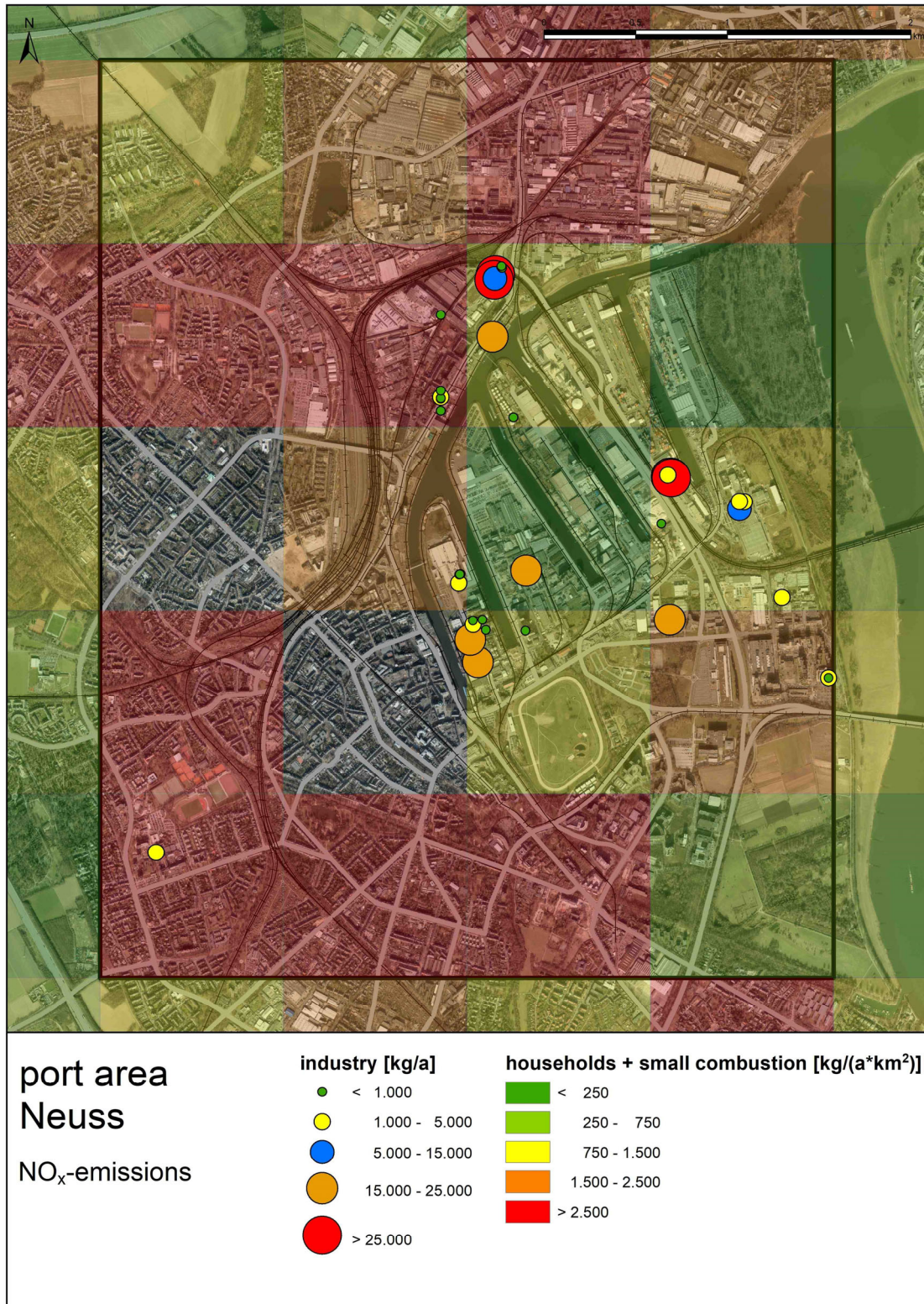
Figure 30: Annual NO x emissions from industrial sources, small combustion plants and domestic furnaces in the Neuss port area, analysis year 2018
