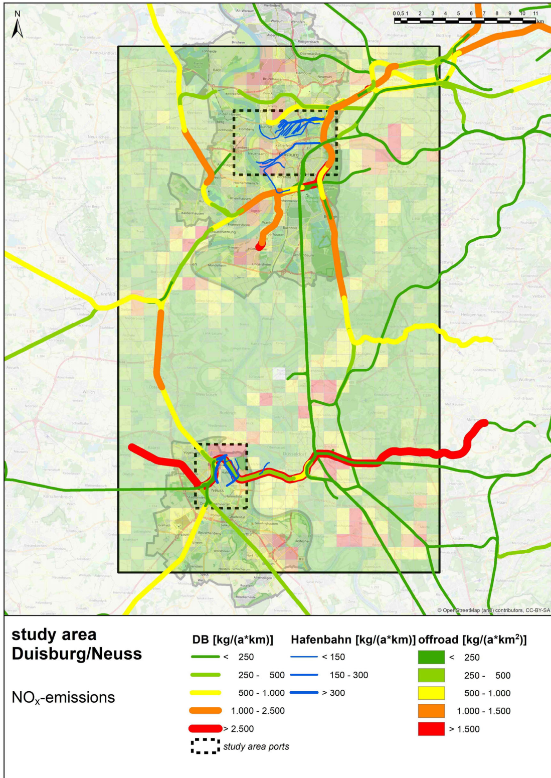
Figure 21: Emissions from rail traffic and off-road in the study area, analysis year 2018
