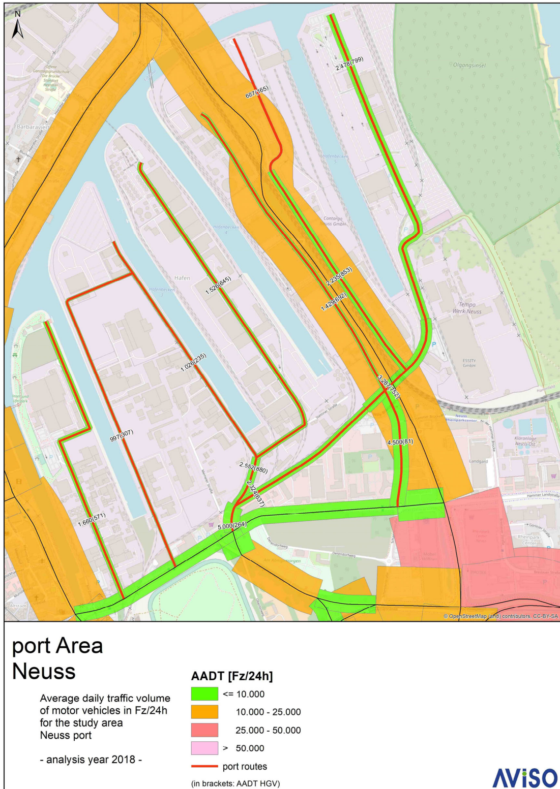
Figure 24: Motor vehicle traffic volumes in the port area for the analysis year 2018 (AADT=daily traffic volume, vehicles per day)
