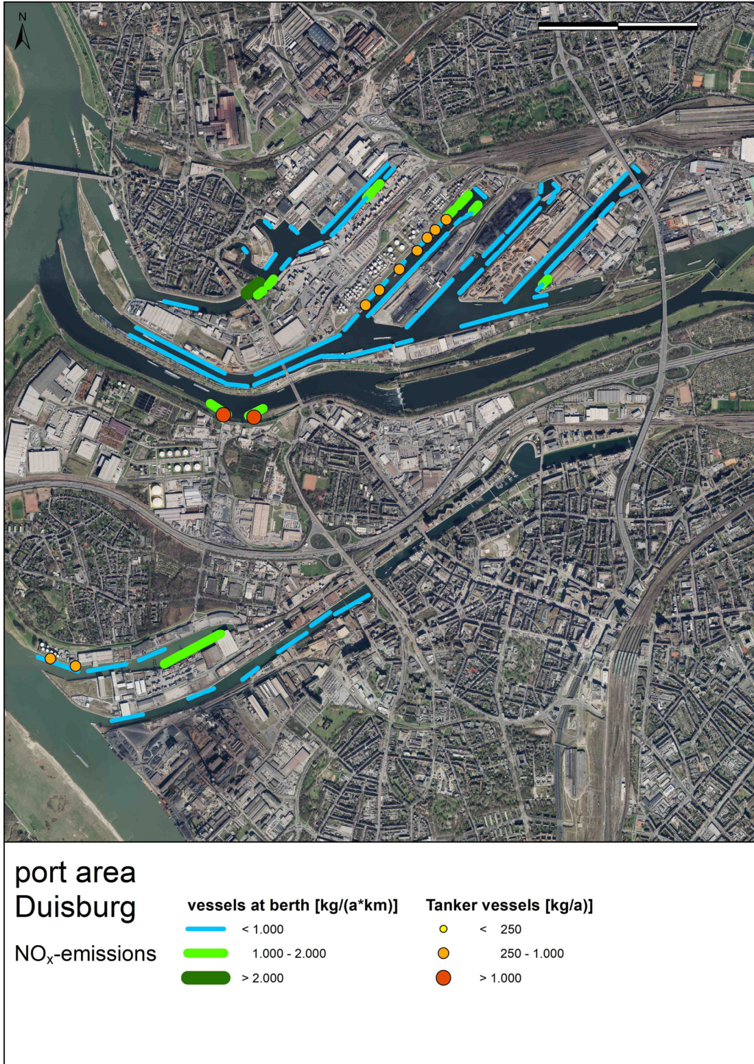
Figure 11: Emissions of moored ships as liner (cargo ships) and point sources (tankers) in the port area of Duisburg
